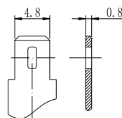
Terminal T1
