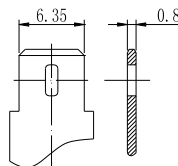
Terminal T2
