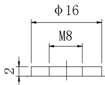
Terminal T11
