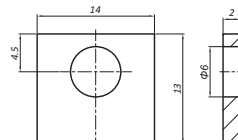
TERMINAL T3
